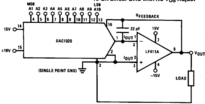
10-Bit Linear DAC with No V_{OS} Adjust
